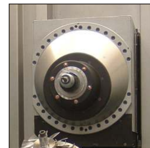
Motorspindle orizzontale Horizontal motorspindle Waagrecht Motorspindel Moteur-brèche horizontale
